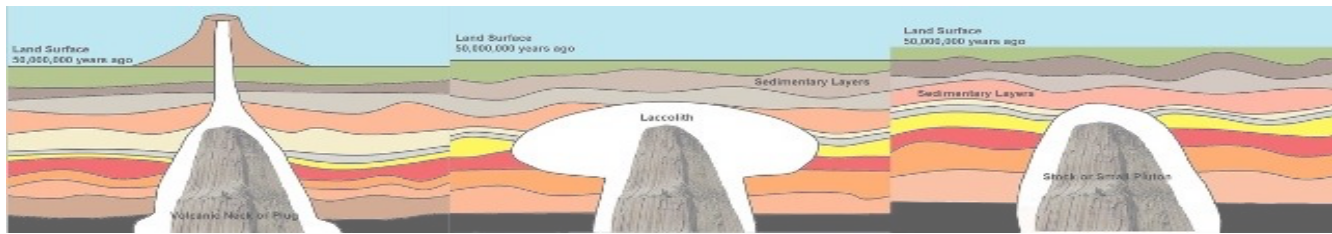
The three Devils Tower formation theories S. Carter
